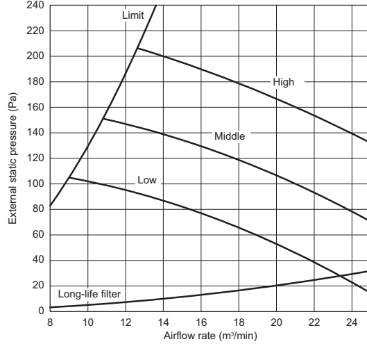
PEFY-P63VMHS-E External static pressure : 100Pa Power source : 220-240V, 50/60Hz
