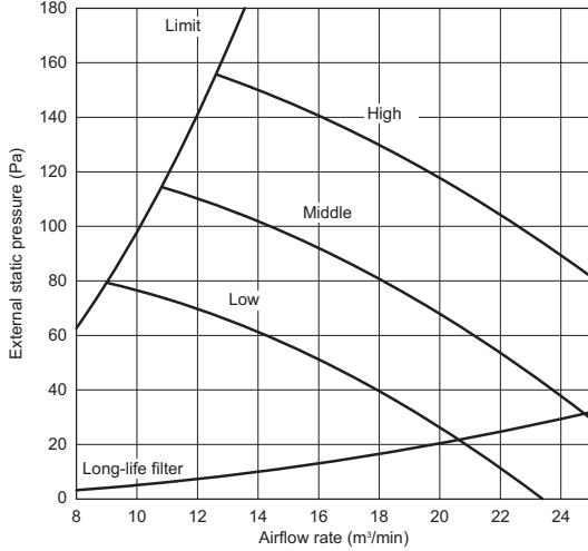
PEFY-P63VMHS-E External static pressure : 50Pa Power source : 220-240V, 50/60Hz
