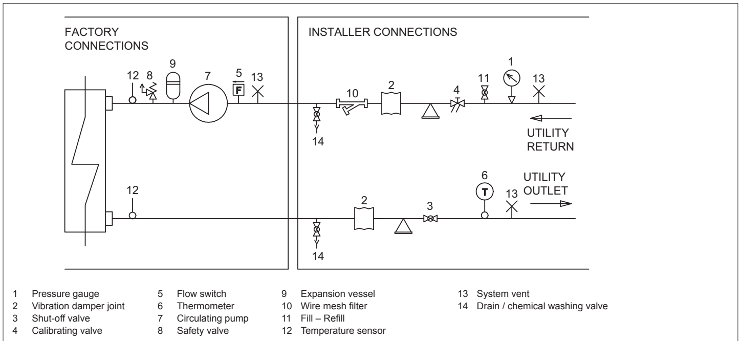
System water circuit connection diagram, i-BX with pump
