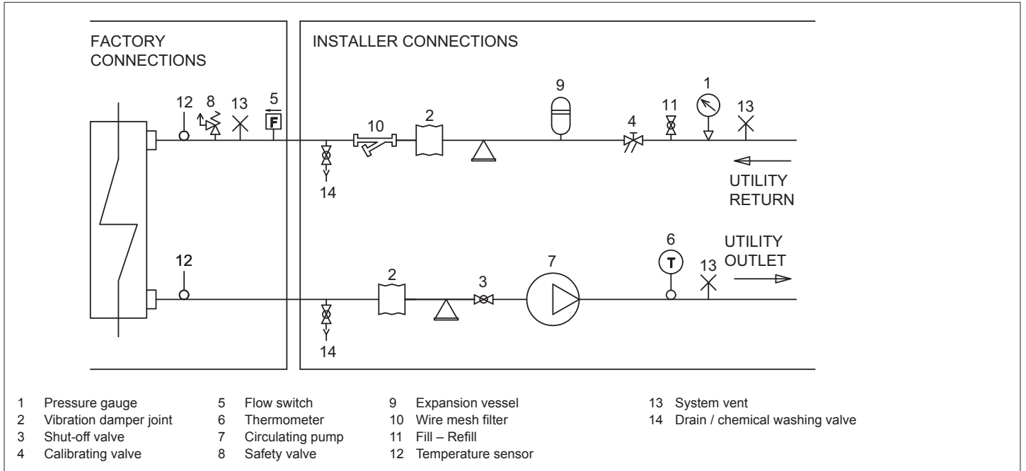
System water circuit connection diagram, i-BX version without pump
