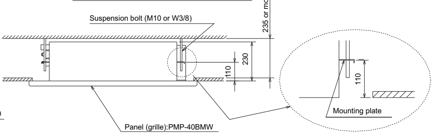
Installation space required around indoor unit
