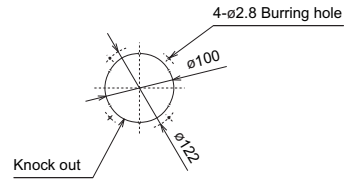
Detail drawing of fresh air intake hole
